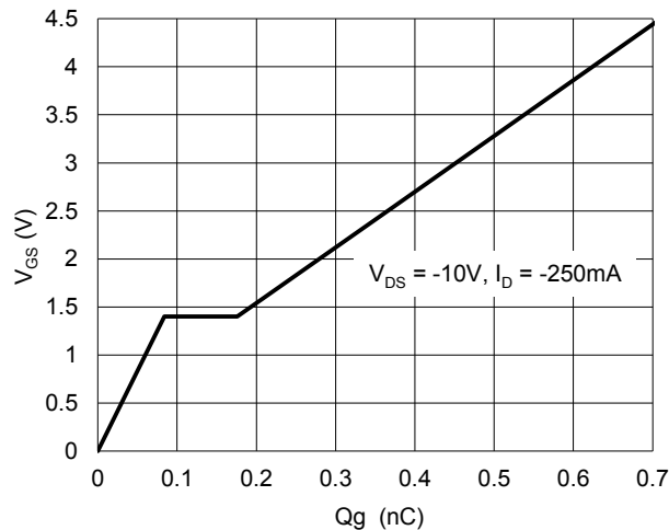
Figure 23. Gate Charge
