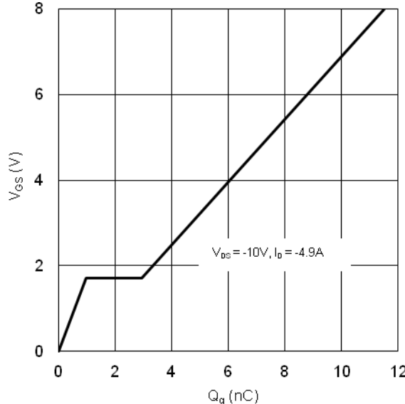
Figure 23 Gate Charge
