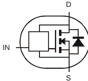
Device Symbol
