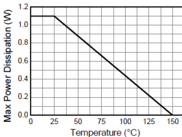
Derating Curve
