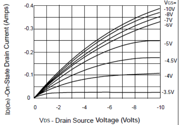
Saturation Characteristics
