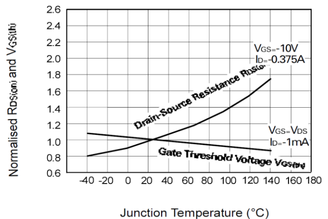
Normalised R_{DS(on)} and V_{GS(th)} vs Temperature
