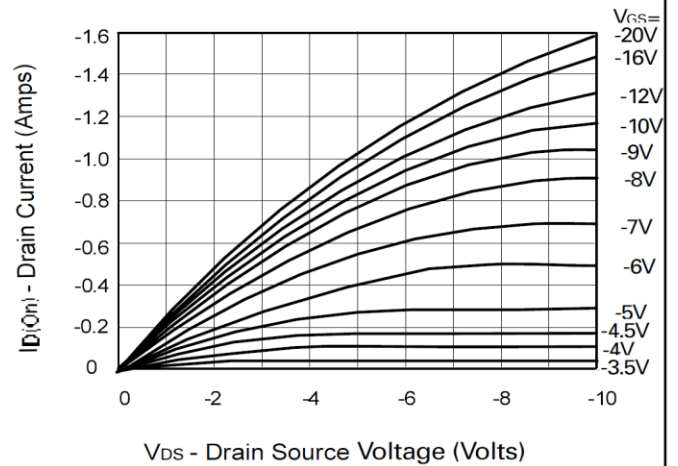
Saturation Characteristics
