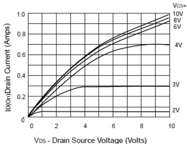
Saturation Characteristics
