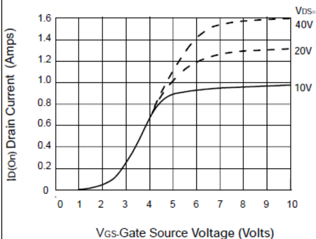
Transfer Characteristics
