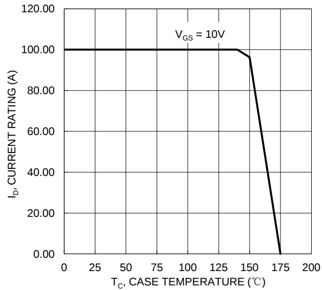
Figure 13. Current De-rating
