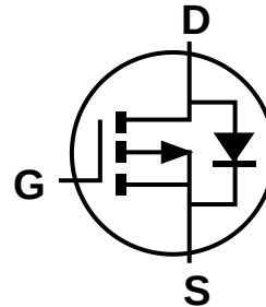
Internal Schematic
