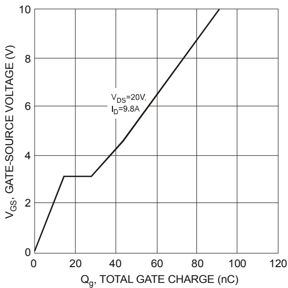
Fig. 11 Gate-Charge Characteristics
