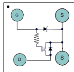
Top View Equivalent Circuit
