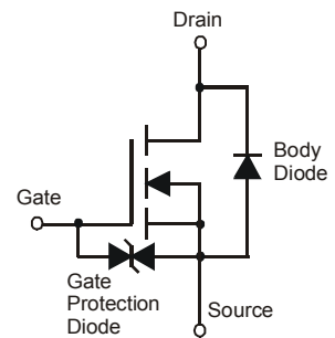
Equivalent Circuit
