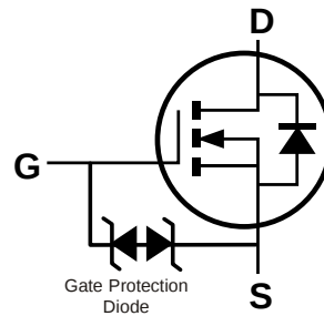
Equivalent Circuit
