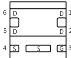
Bottom View Pin Out
