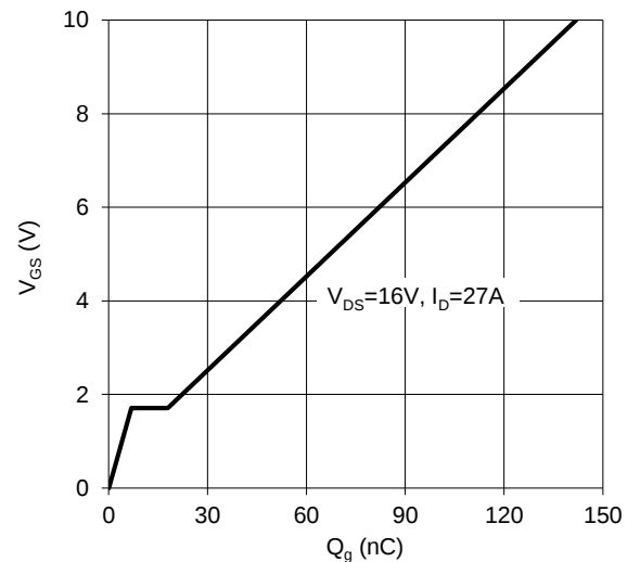
Figure 12. Gate Charge
