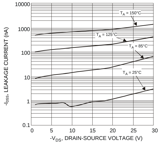
Fig. 10 Typical Drain-Source Leakage Current vs. Voltage
