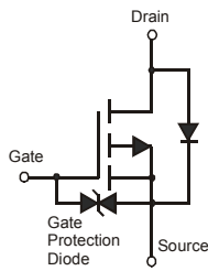
Pinout Circuit
