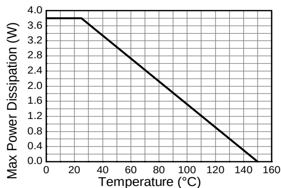
Derating Curve
