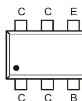
Pin-Out Top
