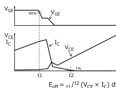
Fig. 6.2.4 Timing Chart of Switching Loss
