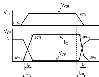
Fig. 6.2.2 Timing Chart of Switching Time
