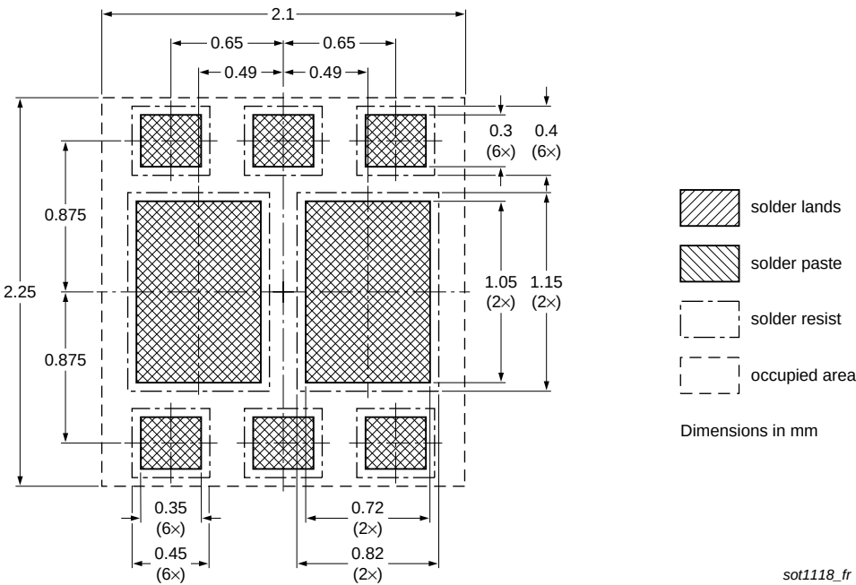
Fig 19. Reflow soldering footprint for SOT1118 (HUSON6)
