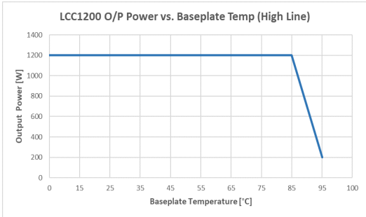
Figure 2. Output Power vs. Baseplate Temperature (180VAC to 264VAC)
