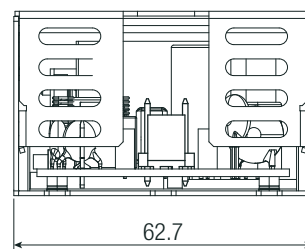
AC Input Side View
