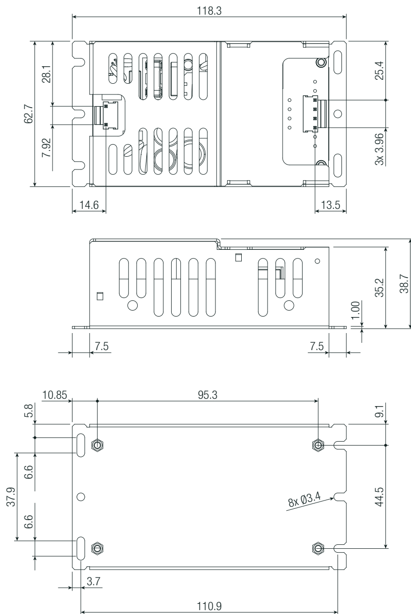
Dimension Drawing “/ENC” (mm)
