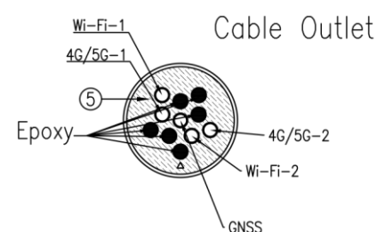
BottomThread View
