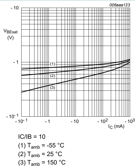
Fig. 10. BC807-25QBH-Q: Base-emitter saturation voltage as a function of collector current; typical values
