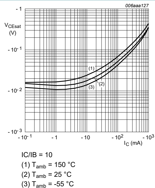
Fig. 15. BC807-40QBH-Q: Collector-emitter saturation voltage as a function of collector current; typical values
