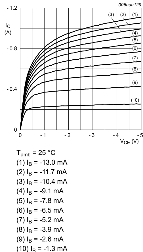
Fig. 9. BC807-25QBH-Q: Collector current as a function of collector-emitter voltage; typical values
