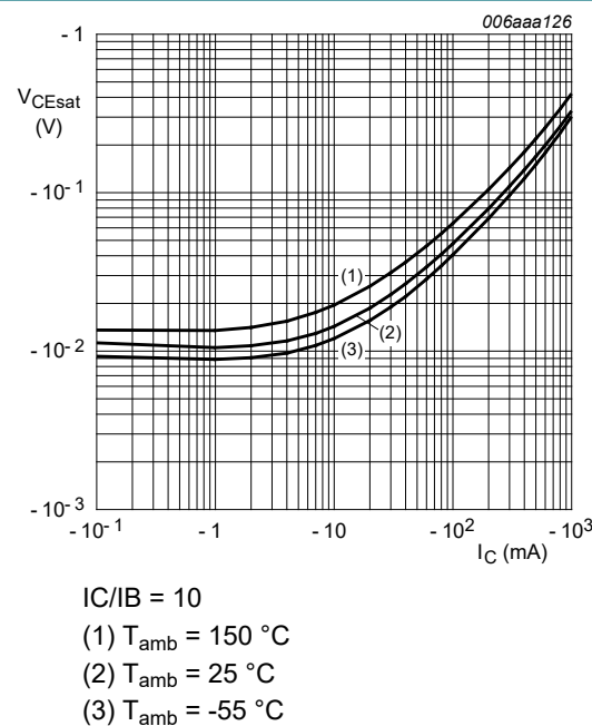
Fig. 11. BC807-25QBH-Q: Collector-emitter saturation voltage as a function of collector current; typical values
