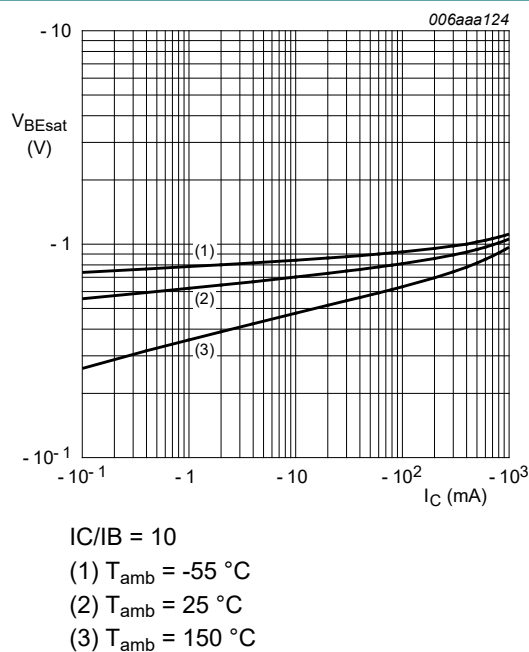
Fig. 14. BC807-40QBH-Q: Base-emitter saturation voltage as a function of collector current; typical values
