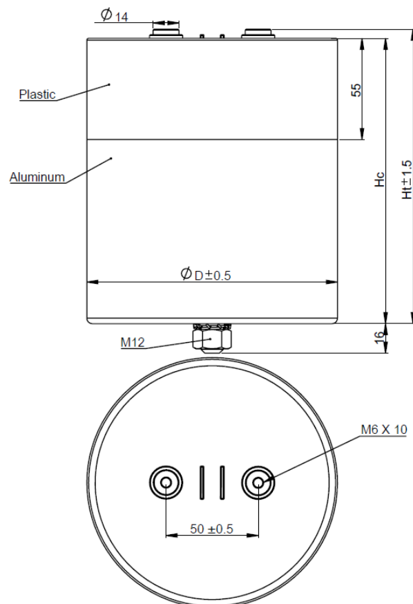
Figure 4: - B25690C - \varnothing D=136 mm - Female terminals (M6) - Between terminals 50 \pm 0.5 mm
