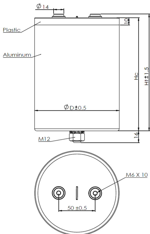
Figure 3: - B25690A - \varnothing D=116 mm - Female terminals (M6) - Between terminals 50 \pm 0.5 mm
