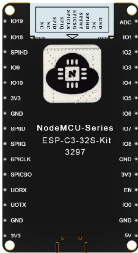
ESP-C3-32S-Kit pin diagram
