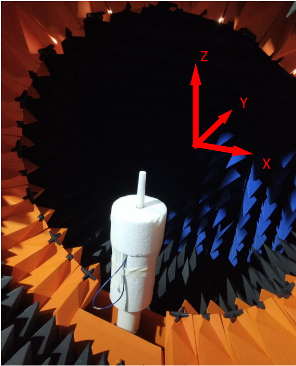
Free space - Antenna 90 degrees
