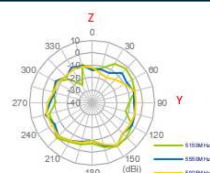
YZ Plane
