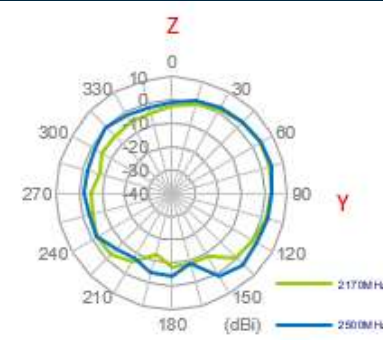
YZ Plane
