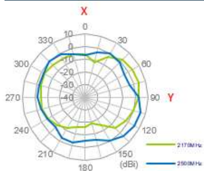
XY Plane
