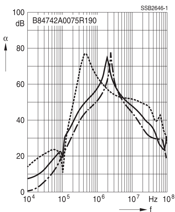
Filters for 75 A
