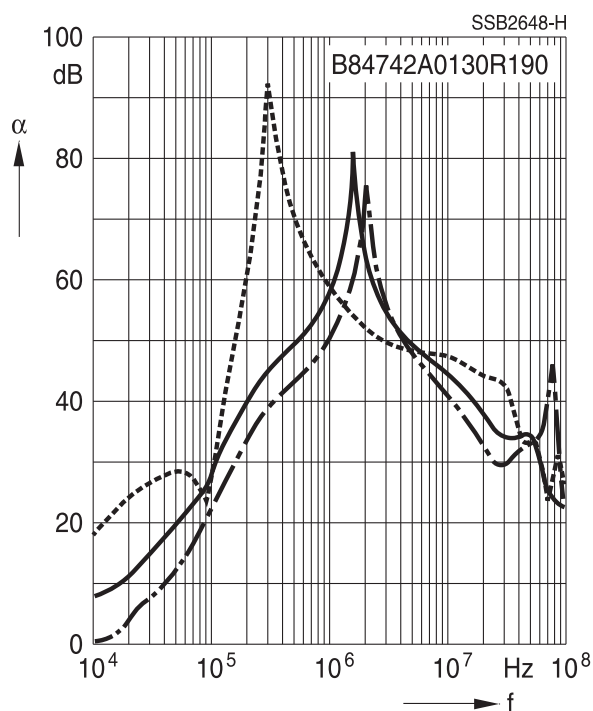
Filters for 130 A
