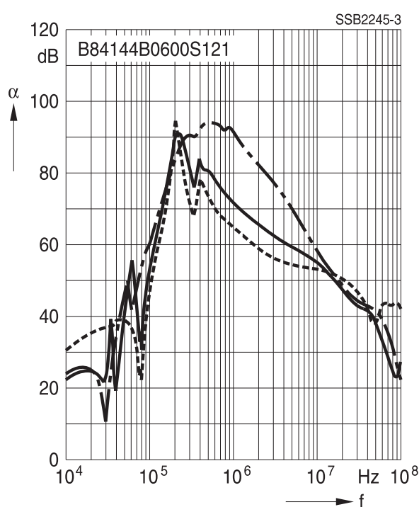
Filters for 600 A (Type S121)
