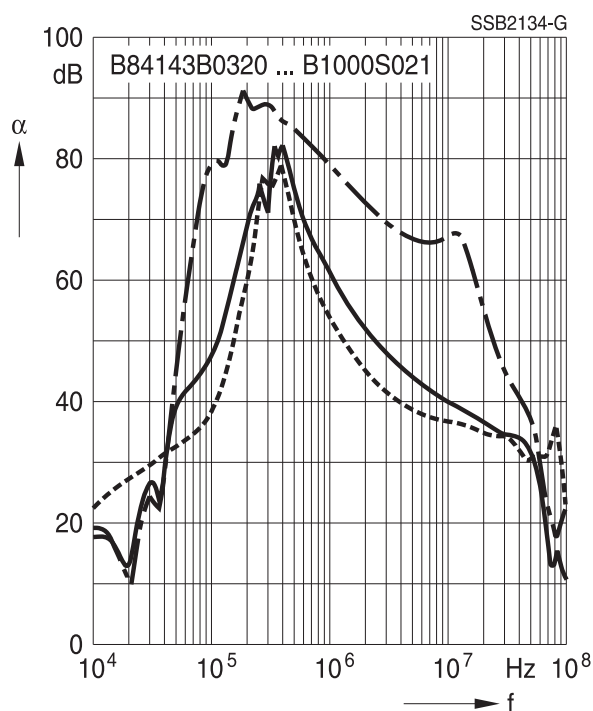
Filters for 320 A ... 1000 A (Type S021)
