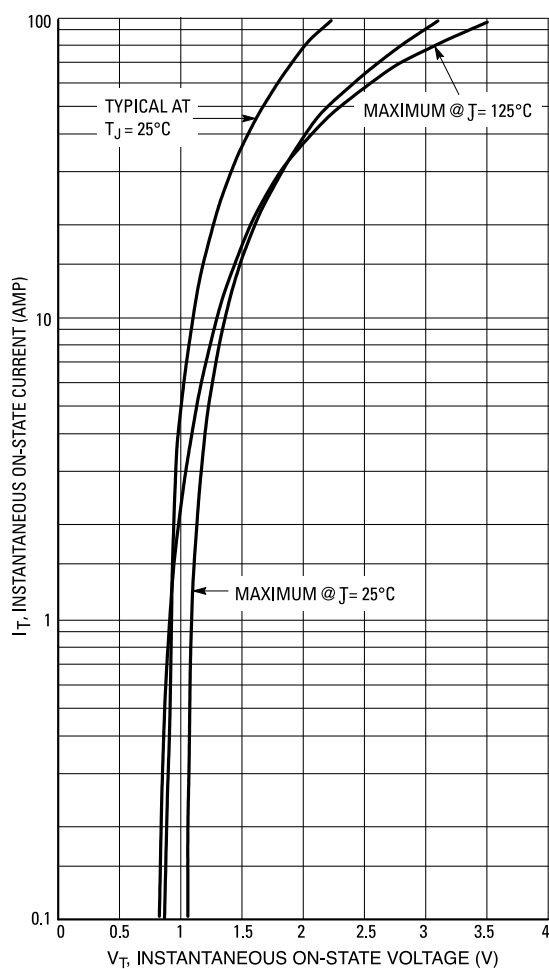
Figure 3. On-State Characteristics
