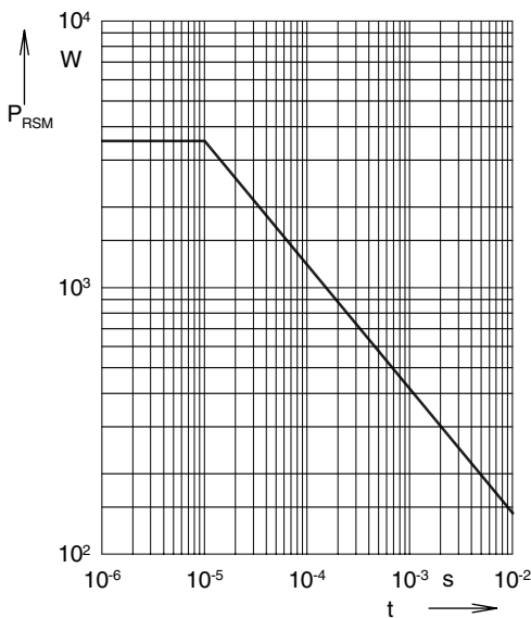
Fig. 3: Power loss
