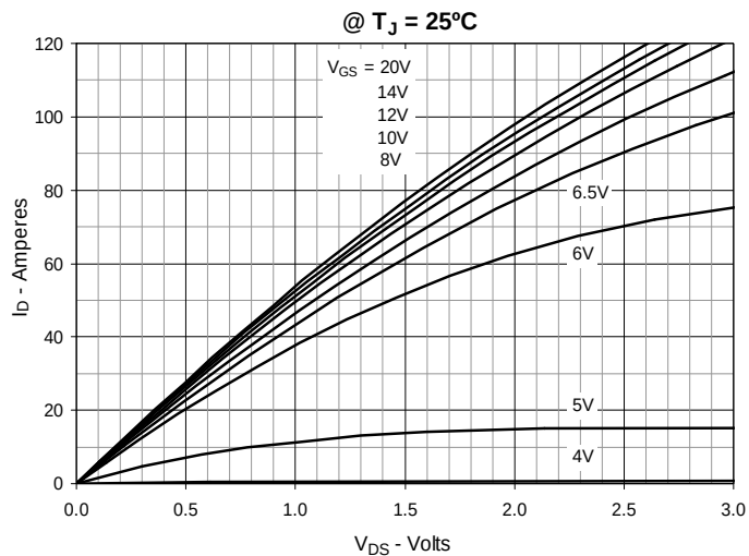
Fig. 1. Output Characteristics
