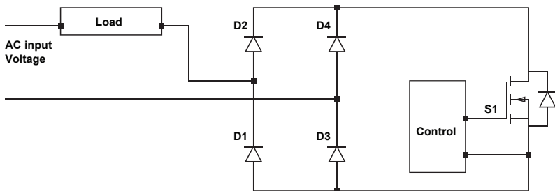
Figure 3: AC switch
