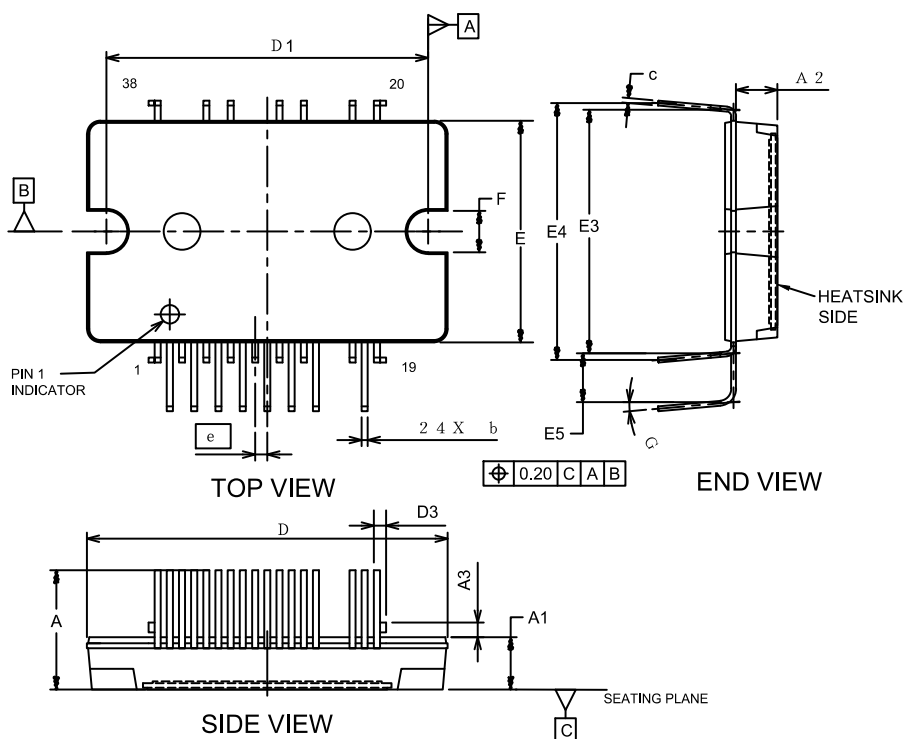
DIP38 29.60x18.20 EP-5 CASE 181AE ISSUE A
