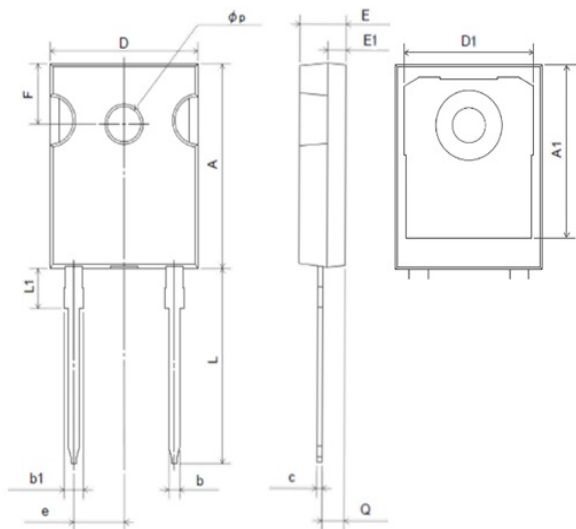
TO-247-2L, (TO-247GE-2L)
