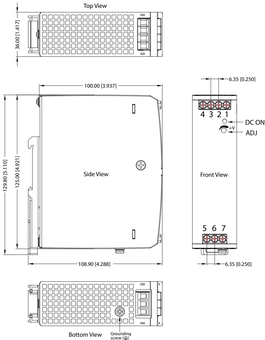
Figure 5. Mechanical Drawing
