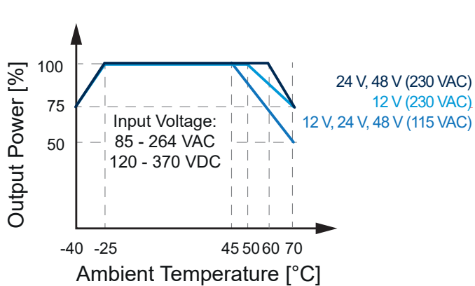
Figure 1. Temperature Derating Curve
