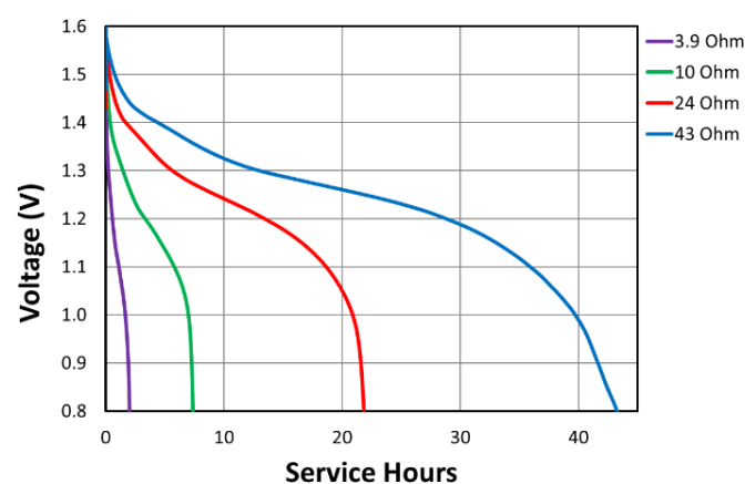
Constant Resistance
