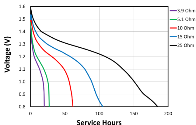
Constant Resistance
