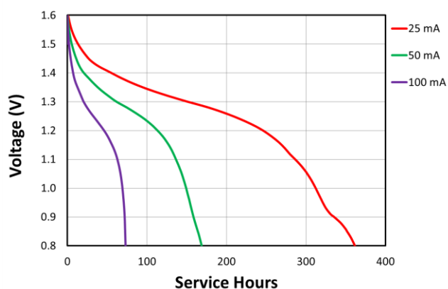
Constant Current
