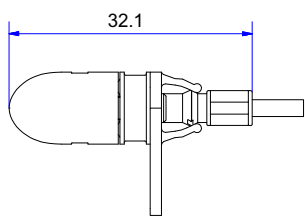
Figure 4 AFBR-S10PS010Z and AFBR-S10PSZ Assembled
