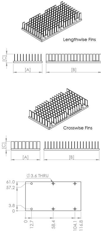
Drawing A: 1/1 Brick geometry
