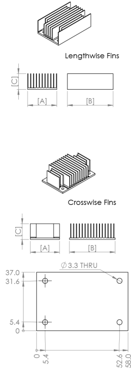
Drawing C: 1/4 Brick geometry
