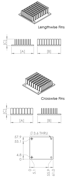
Drawing B: 1/2 Brick geometry
