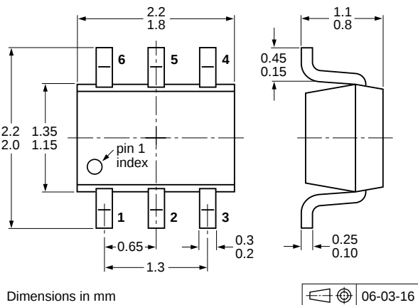
Fig 11. Package outline PUMH15 (SOT363)
