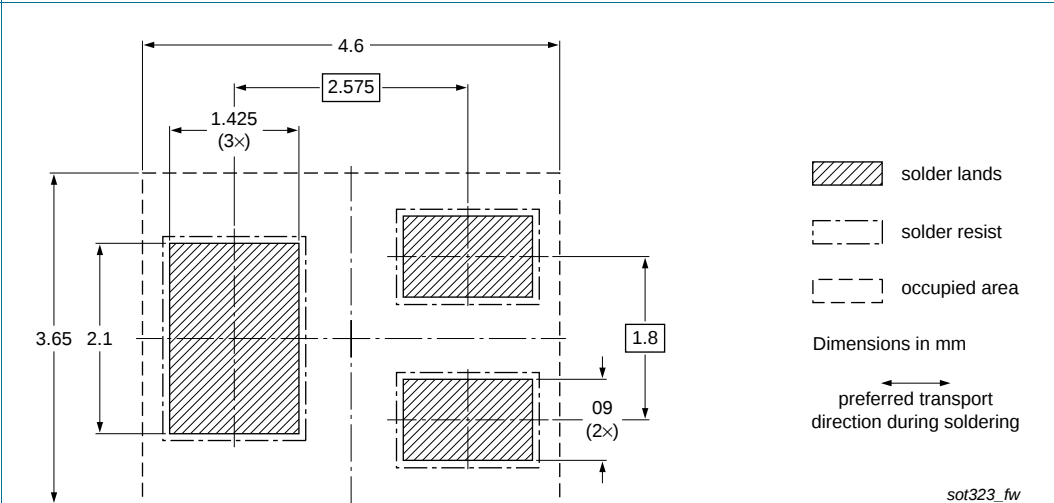
Fig 20. Reflow soldering footprint PDTC144EU (SOT323/SC-70)
