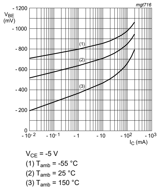
Fig. 7. BC857BW-Q: Base-emitter voltage as a function of collector current; typical values
