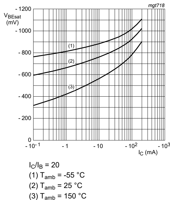
Fig. 9. BC857BW-Q: Base-emitter saturation voltage as a function of collector current; typical values
