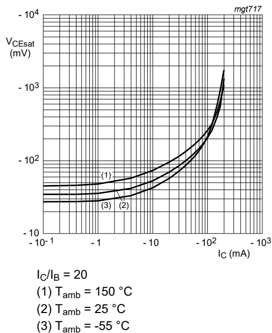
Fig. 8. BC857BW-Q: Collector-emitter saturation voltage as a function of collector current; typical values
