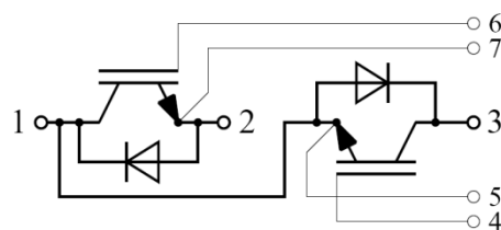
Equivalent Circuit Schematic
