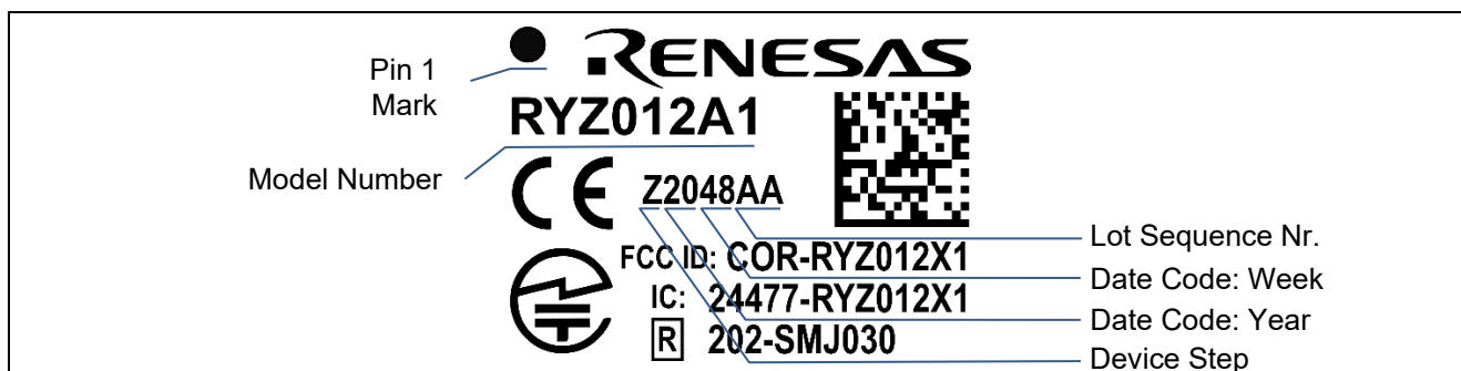
Figure 5. Marking diagram
