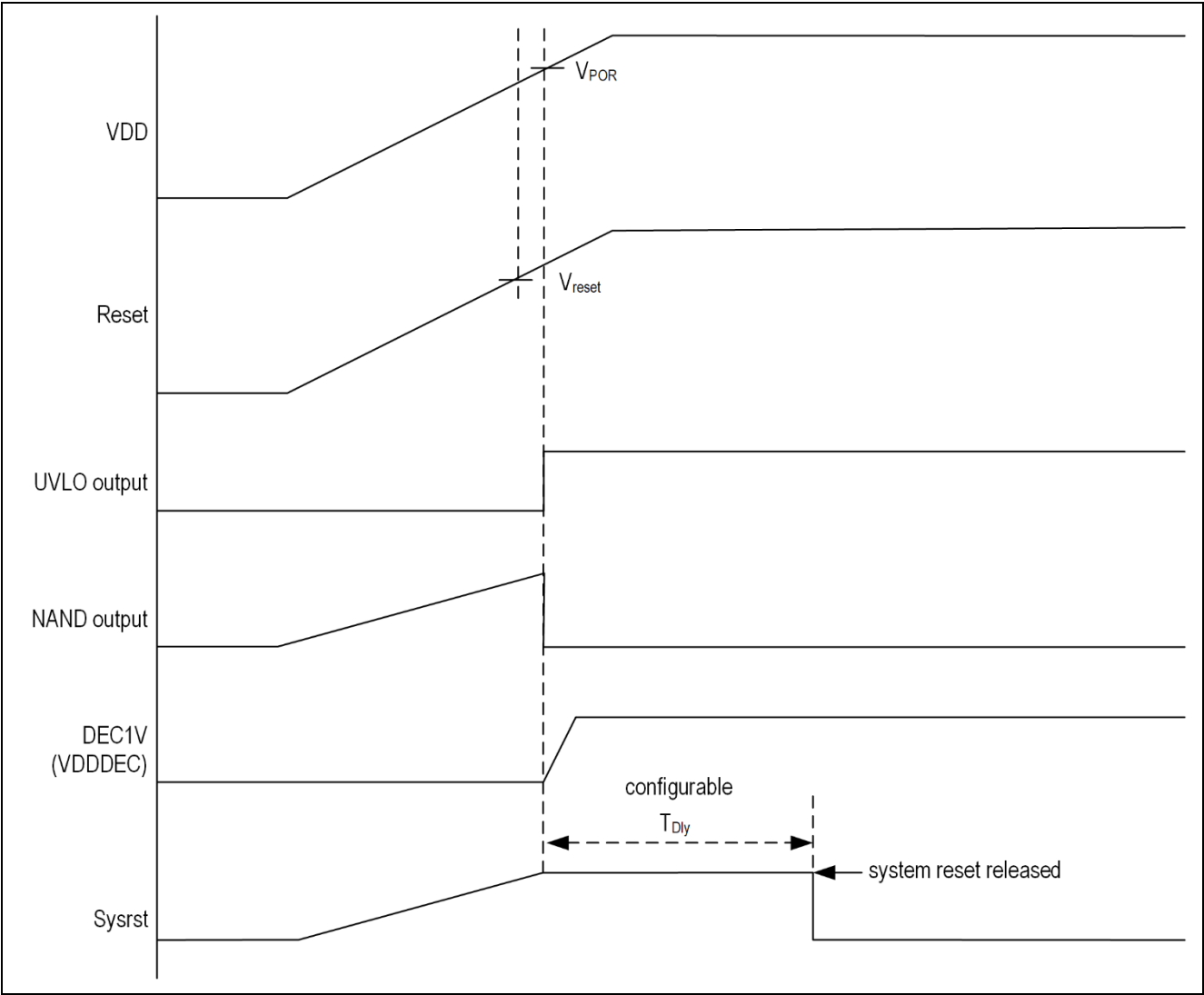
Figure 2. Power-up sequence
