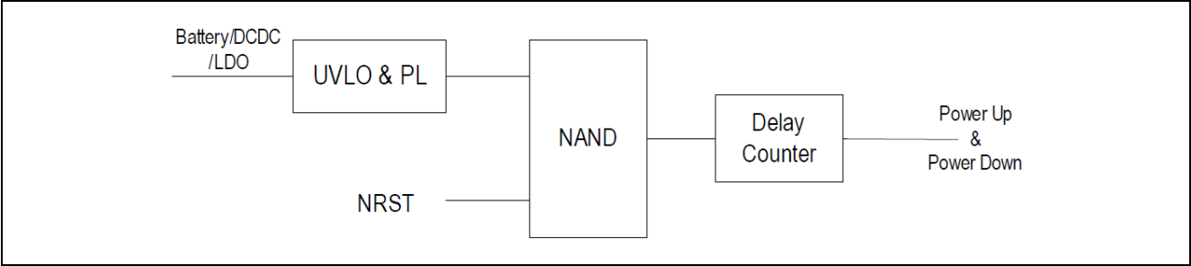
Figure 1. Power control logic
