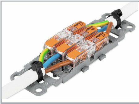
3-pole mounting carrier with strain relief
